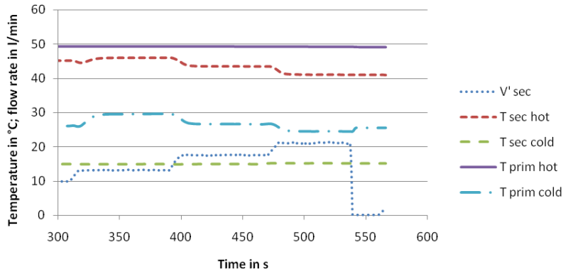
Figure 2 Example for a measurement of the maximum flow rate. The DHW temperature is set to 45°C, the primary inlet temperature to 50°C and the secondary inlet to 15°C. Then the flow rate is increased until the secondary hot temperature drops below 42°C.
