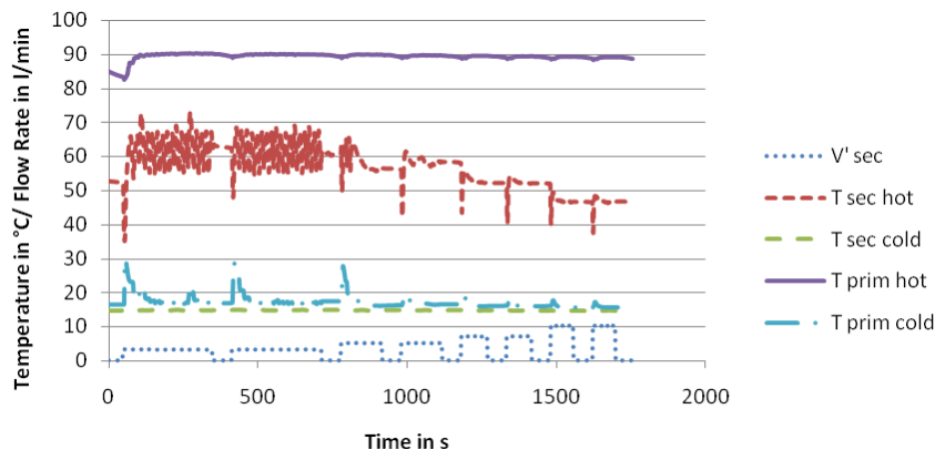
Figure 4 Example of a measurement with small flow rates where three different phenomena are visible: 1. At the flow rate of 3 l/min the temperature of the provided tap water (Tsec hot) oscillates, 2. This temperature decreases with an increasing flow rate. 3. Over-/undershoots occur at the beginning of each draw off.
